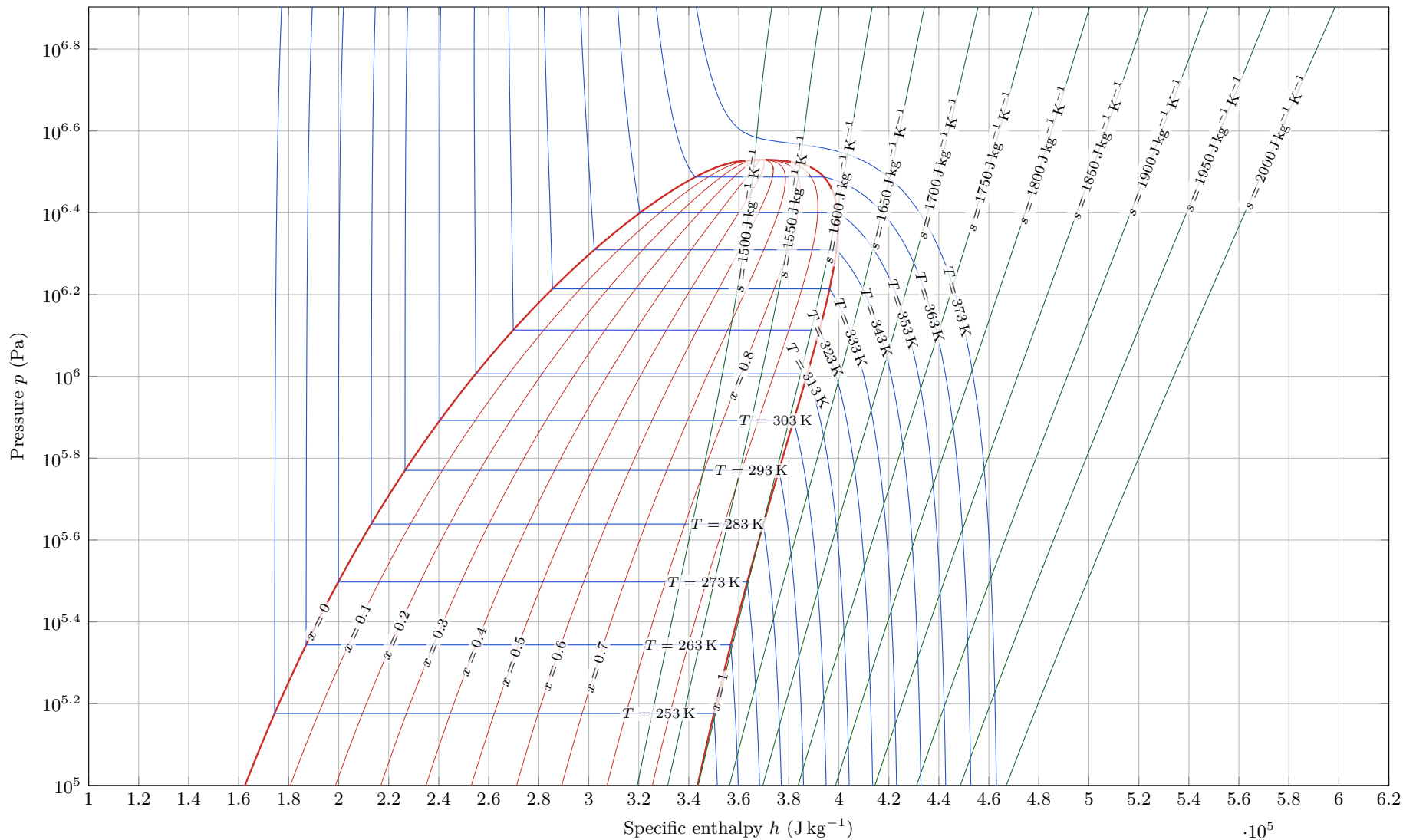
R1234yf pressure–enthalpy diagram
