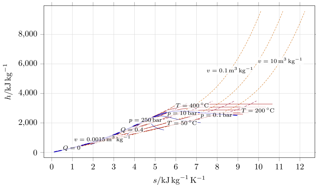
Water enthalpy–entropy diagram
